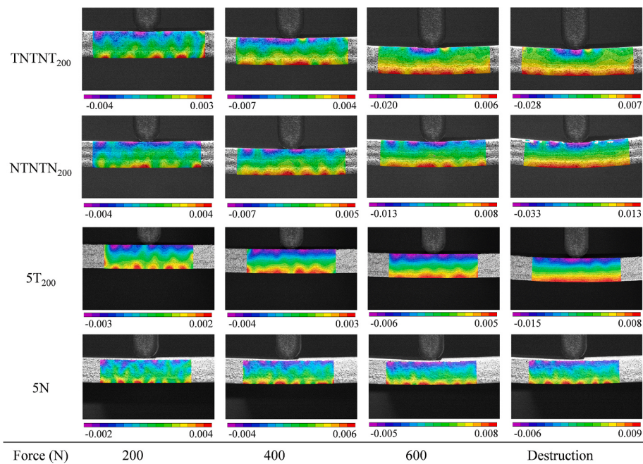
Fig. 5. \varepsilon_{xx} contours of plywood composed of fully and partially 200 °C heat-treated veneers at various load levels.
