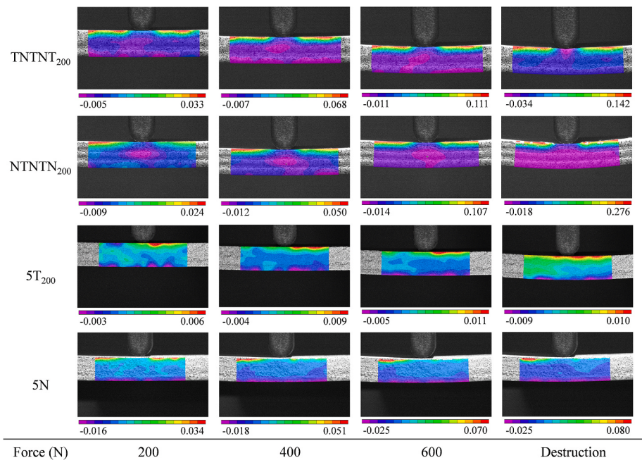
Fig. 6. \varepsilon_{yy} contours of plywood composed of fully and partially 200 °C heat-treated veneers at various load levels.
